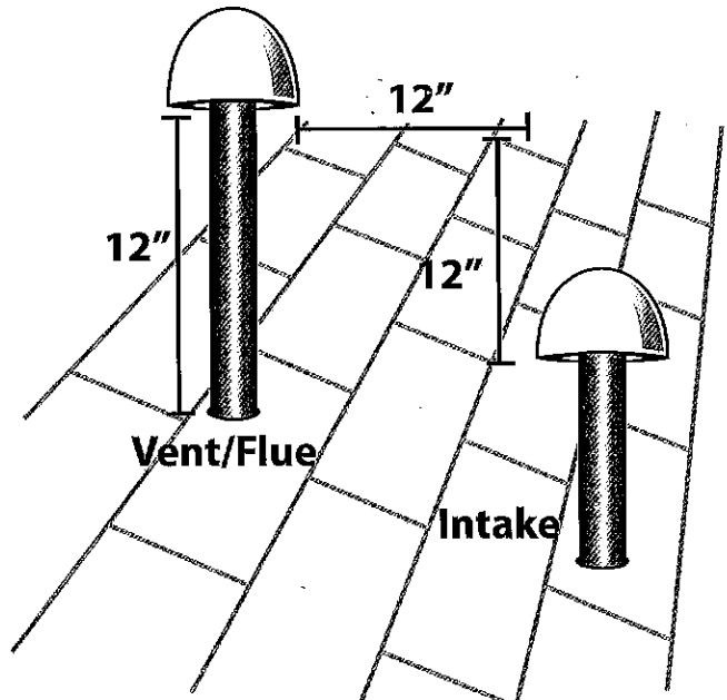
Vertical Termination (Dual Pipe)
