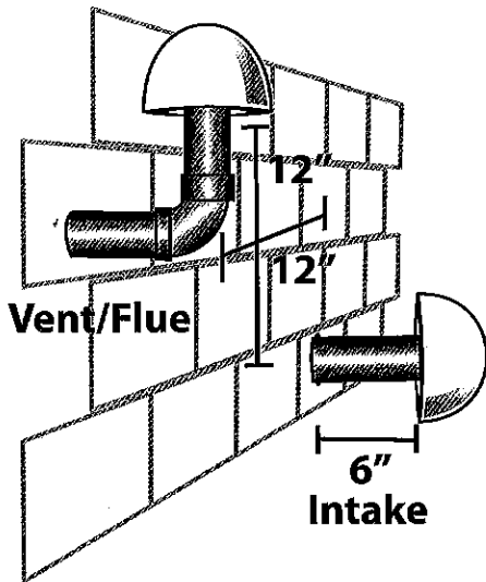
Horizontal Termination (Dual Pipe)
